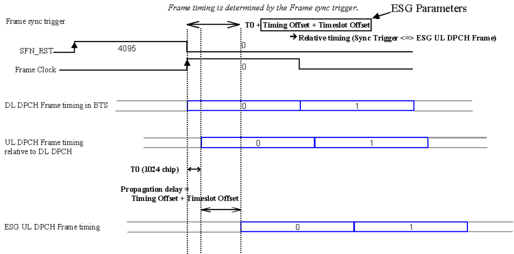
Figure 16-79 DPCH Synchronization - Frame Timing Alignment
