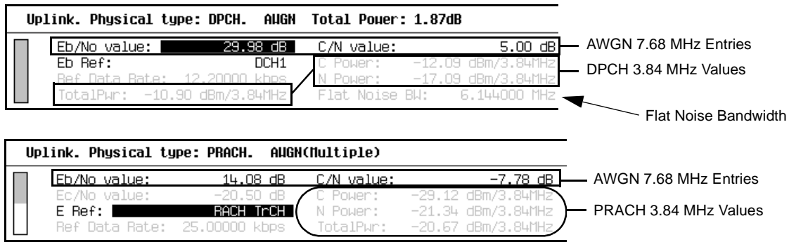
Figure 16-87 Noise Measurement Bandwidths
