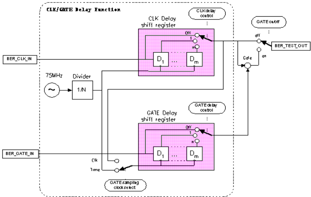
Figure 9-20 Signal Flow
