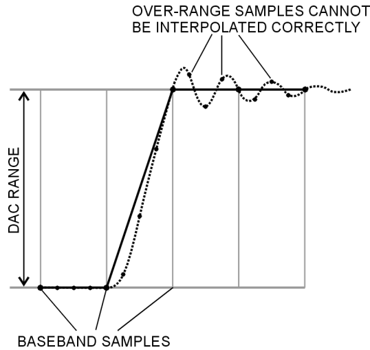
Figure 4-25 Waveform Overshoot
