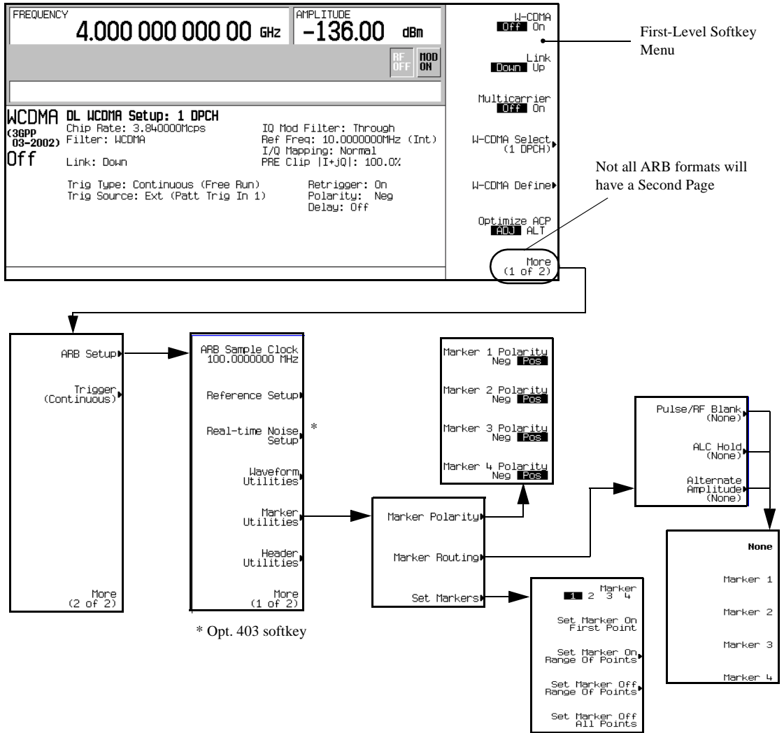
Figure 4-15 ARB Marker Location and Softkey Menus
