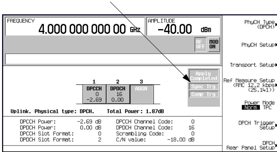
Figure 16-85 Front Panel Display Synchronization Annunciator
