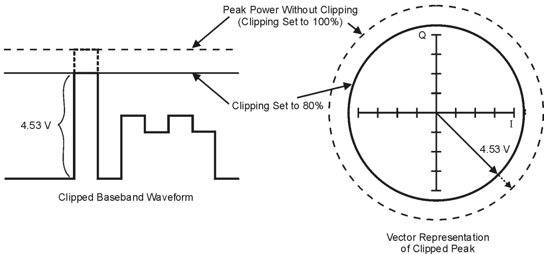
Figure 4-21 Circular Clipping
