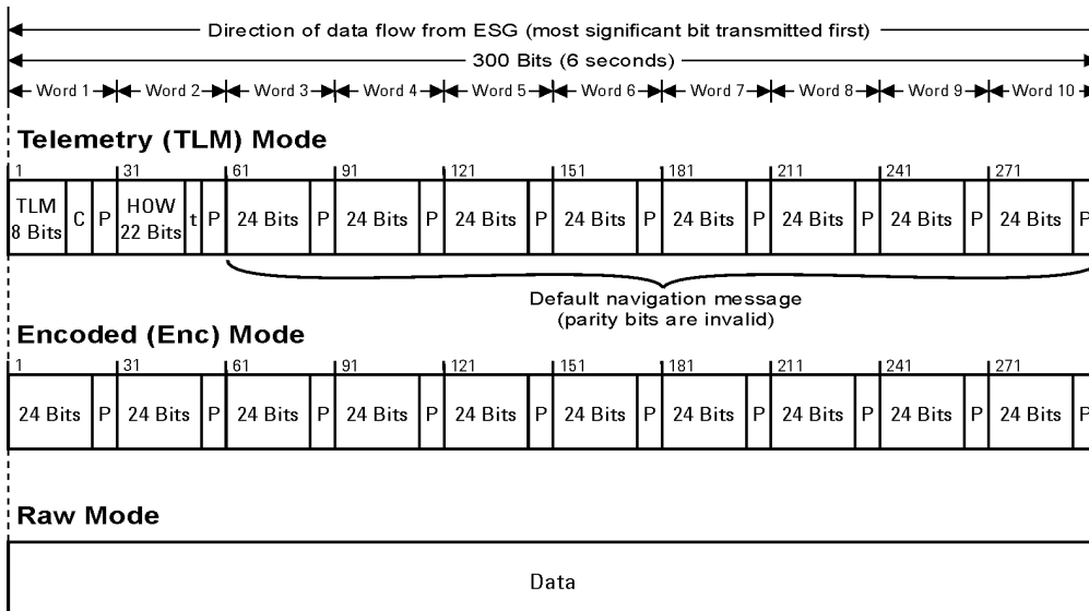
Figure 11-2 Subframe Structures
