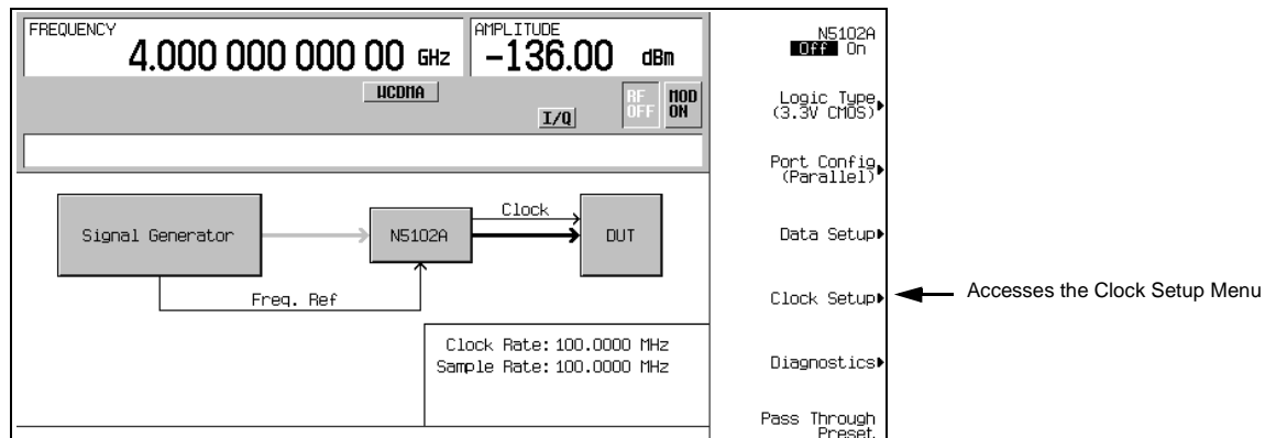
Figure 7-13 Clock Setup Menu Location
