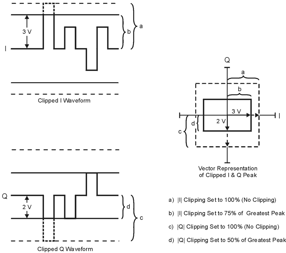
Figure 4-22 Rectangular Clipping
